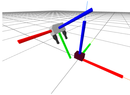
Figure 3.5 - The gripper frame and the object frame. For each frame, the positive x axis is in red , the positive y axis is in green , and the positive z axis is in blue (XYZ \Leftrightarrow RGB).
