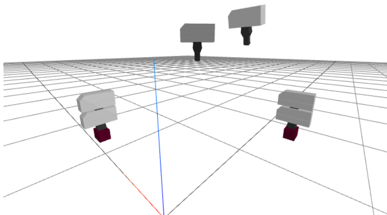
Figure 3.7 - Keyframes of the gripper. The robot's base will be at the origin, so we're looking over the (invisible) robot's shoulder here. The hand starts in the "initial" pose near the center, moves to the "prepick" to "pick" to "postpick" to "clearance" to "preplace" to "place" and finally back to "postplace".
