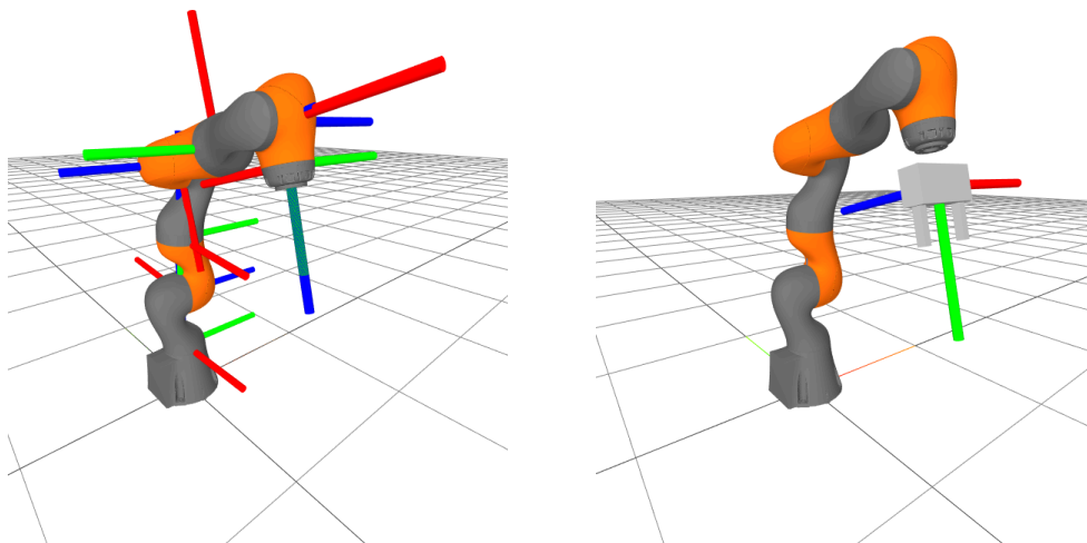
Figure 3.3 - Kinematic frames on the iiwa (left) and the WSG gripper (right). For each frame, the positive x axis is in red , the positive y axis is in green , and the positive z axis is in blue . It's (hopefully) easy to remember: XYZ \Leftrightarrow RGB.
