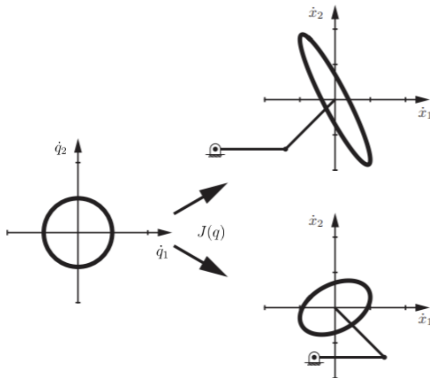
Figure 3.12 - Manipulability ellipsoids for two different postures of the planar two-link manipulator. Adapted from [3].
